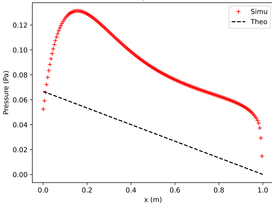
Pressure profile it= 233
