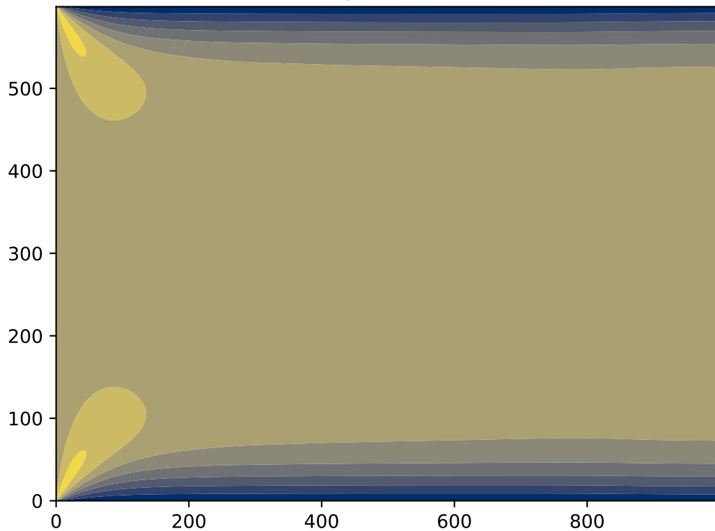
Velocity field it= 573
