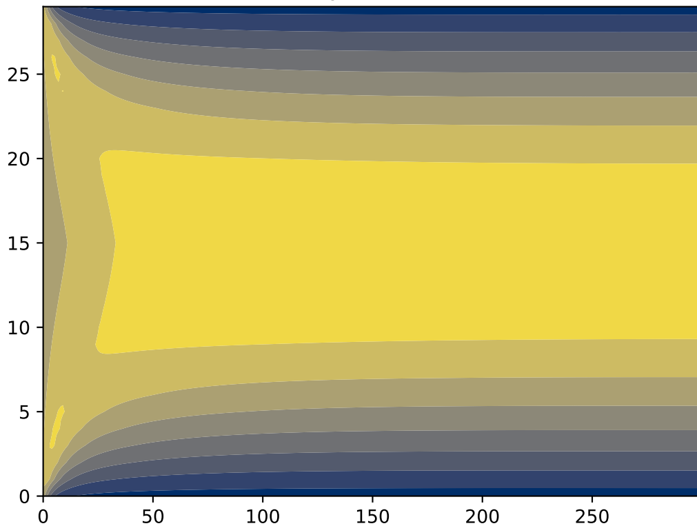
Velocity field it= 641
