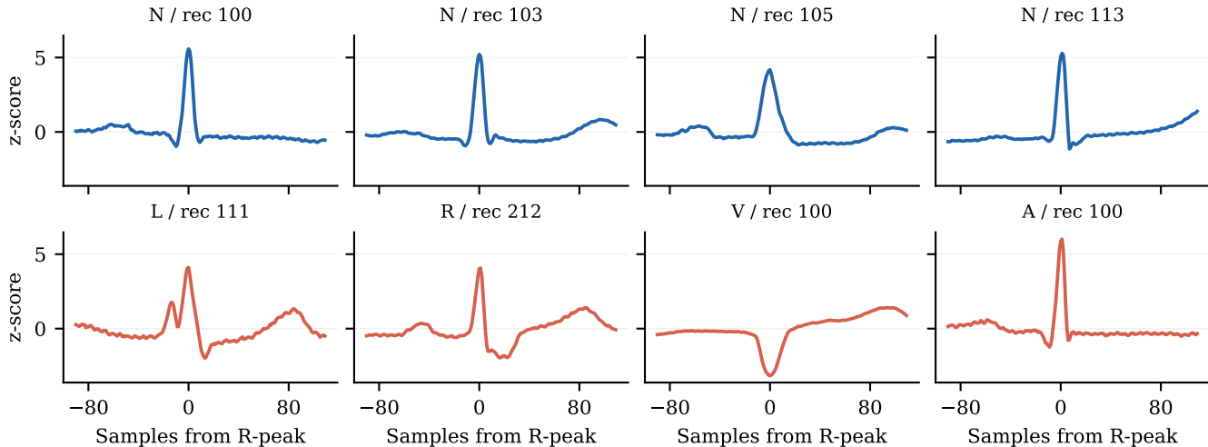
MIT-BIH beat windows: normal (top) and abnormal (bottom)
