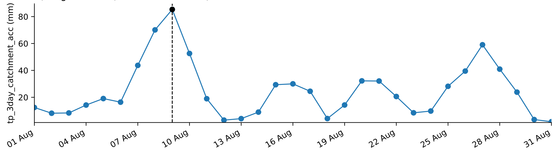
C) Event return period \approx 520.4 years
