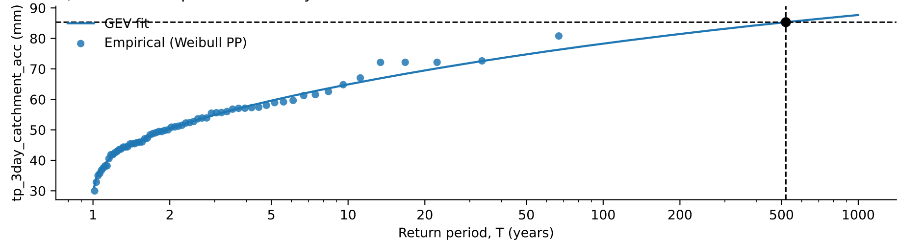
C) Event return period \approx 520.4 years
