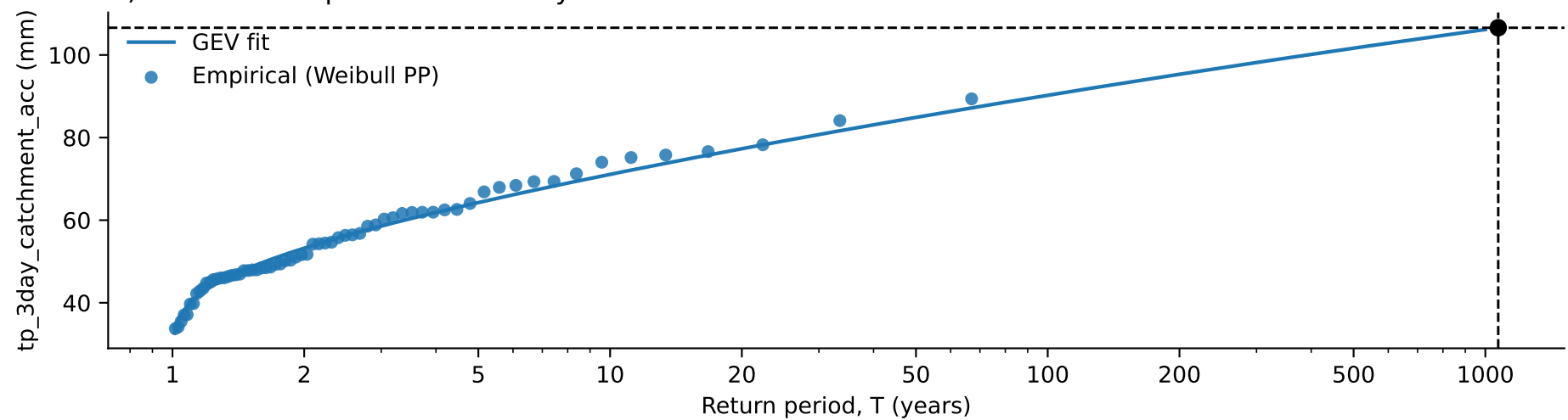
C) Event return period \approx 1070.1 years
