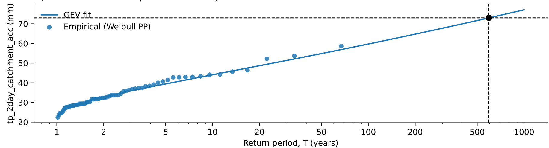
C) Storm Hans return period \approx 594.5 years
