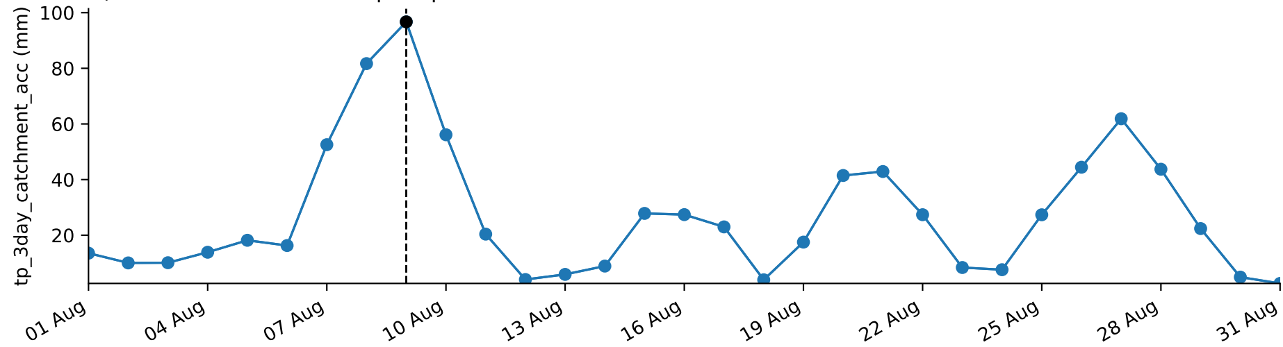
C) Storm Hans return period \approx 950.1 years
