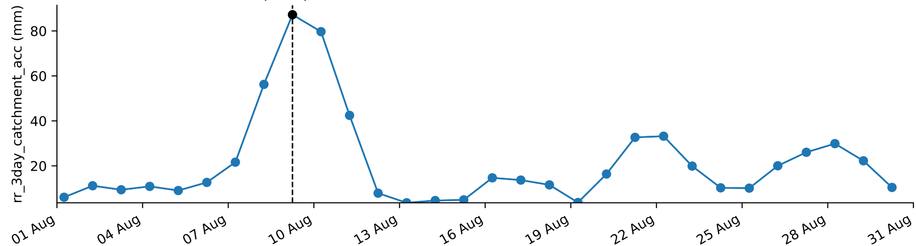
C) Storm Hans return period \approx 566.9 years
