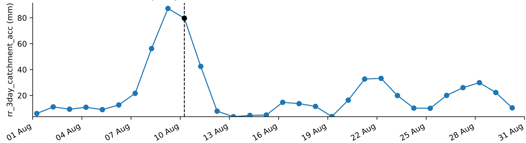
C) Storm Hans return period \approx 254.2 years
