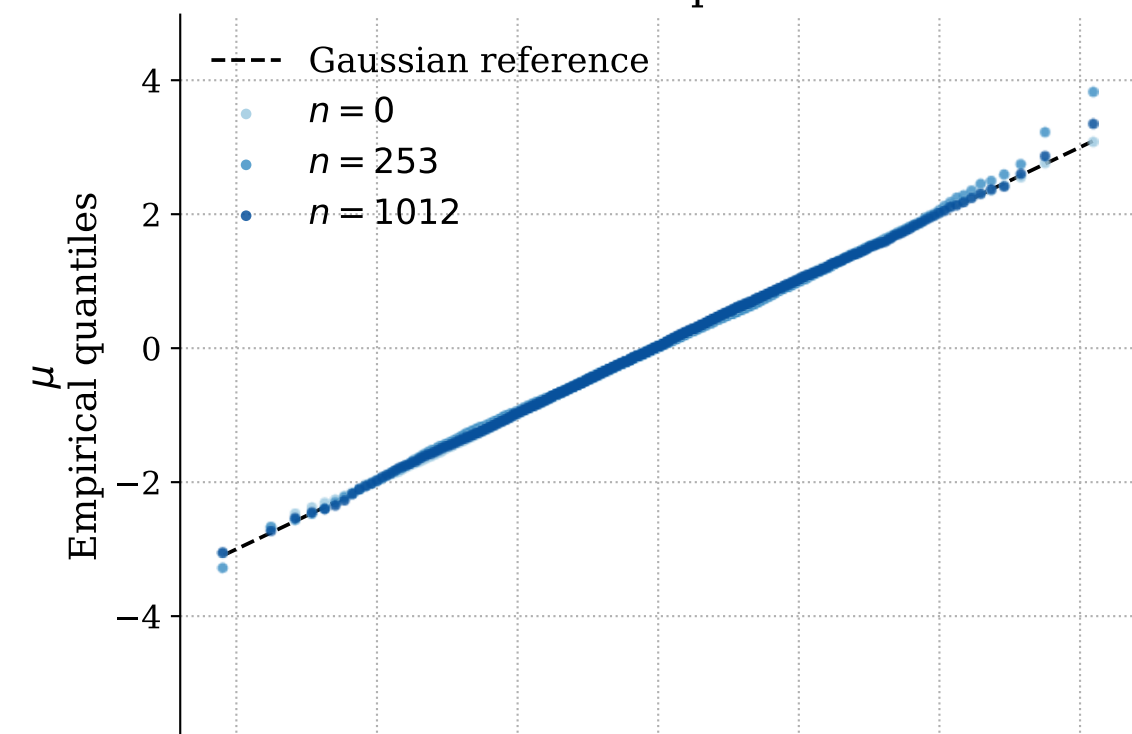
Default prior
