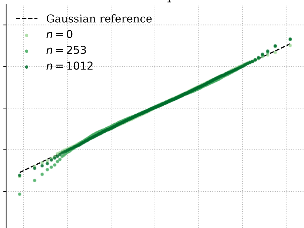
Finance prior
