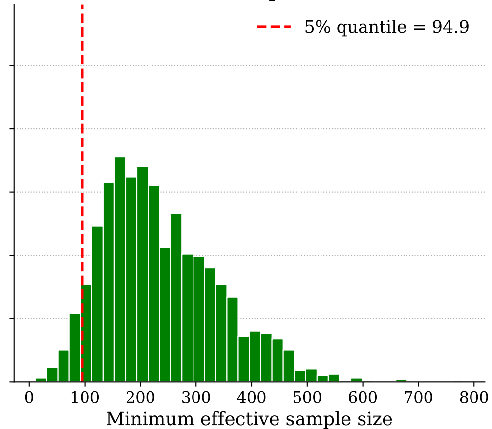
Finance prior
