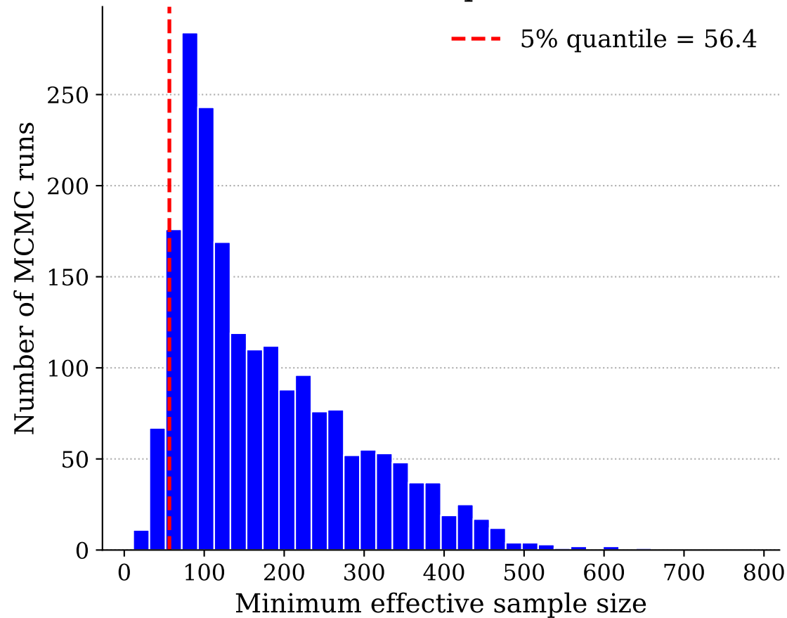
Default prior
