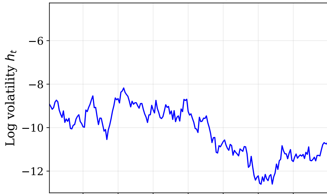
Gaussian innovations ( \nu = \infty, r = 0 )
