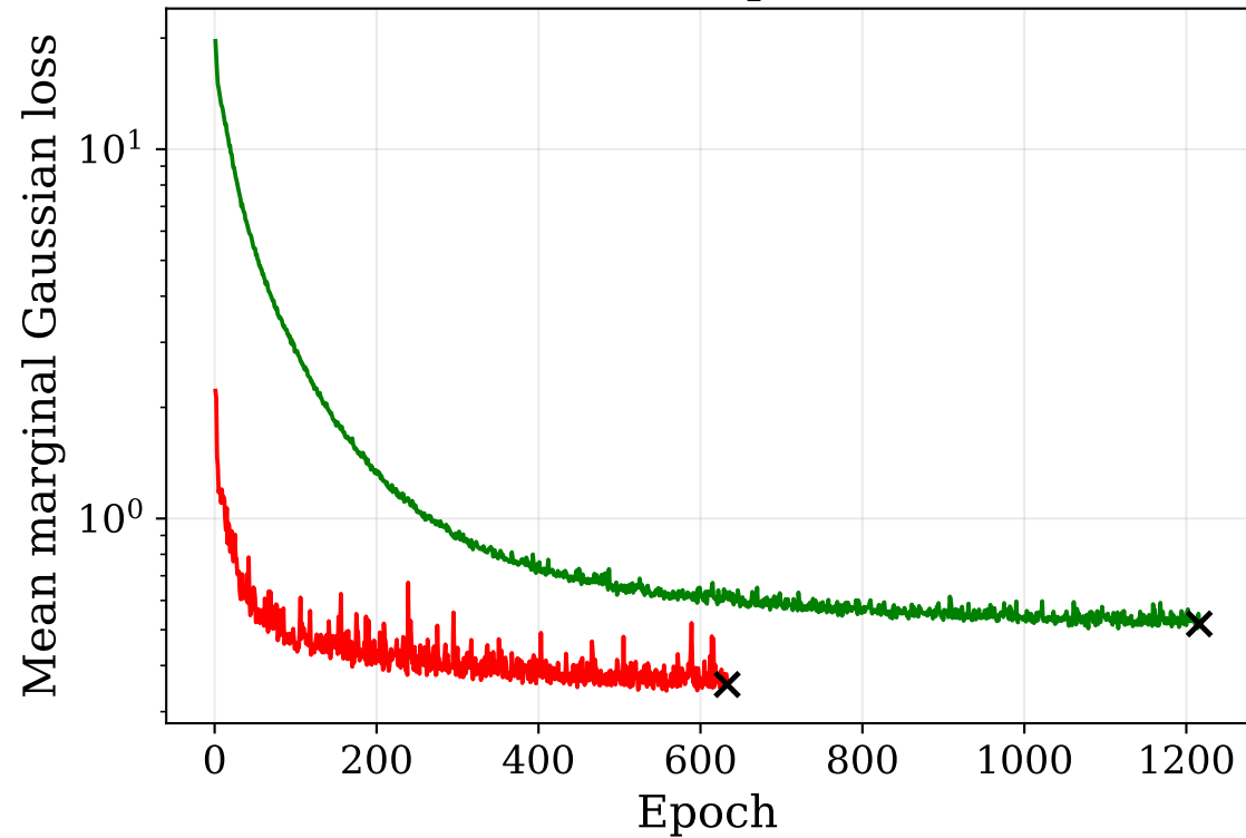
Default prior
