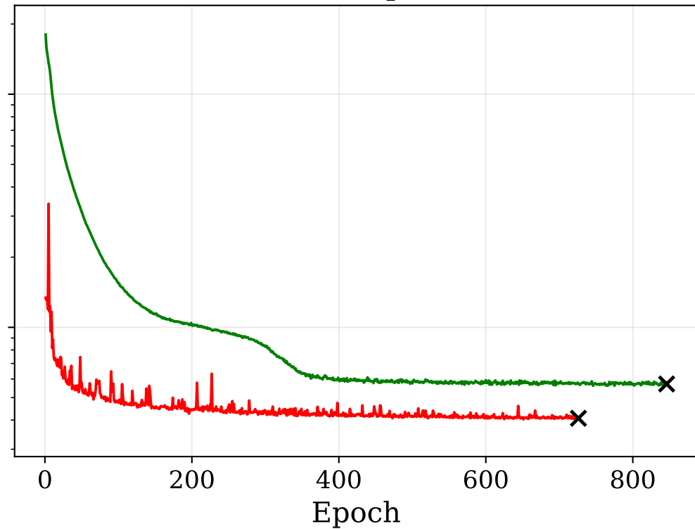
Finance prior
