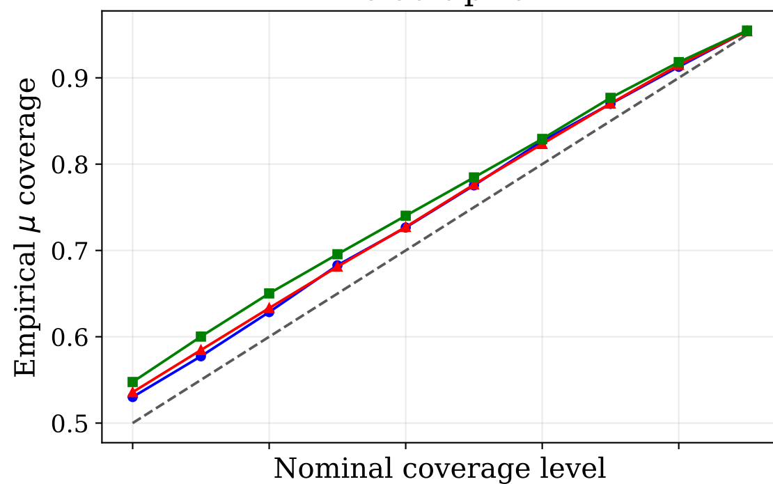
Default prior
