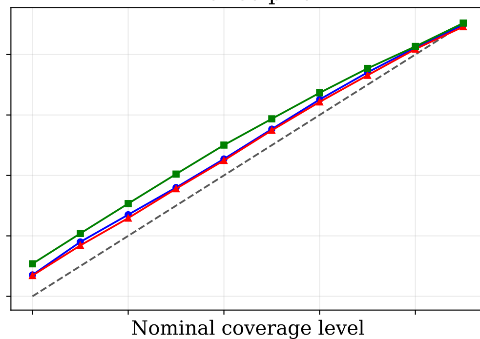
Finance prior
