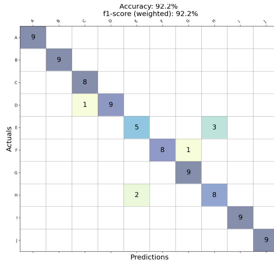
Test confusion matrix
