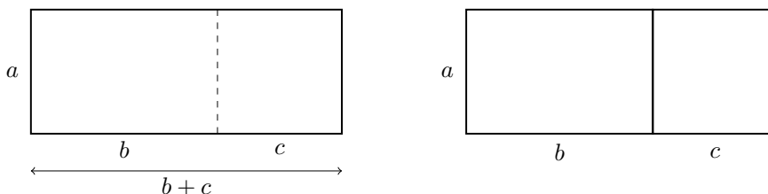
Figure 1.1.65 A picture of a(b + c) and ab + ac
