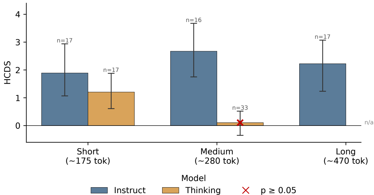
Length-matched HCDS by output-length tier (GSM8K, n=50)
