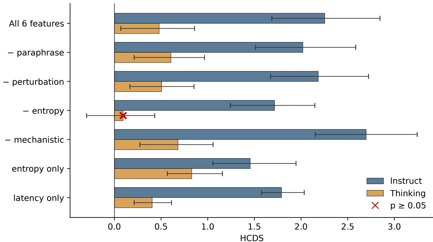
Robustness across HCDS feature subsets (GSM8K, n=50)
