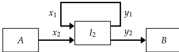
Figure 4.10: An example illustrating that the two-input, two-output identity function is not sequential.
