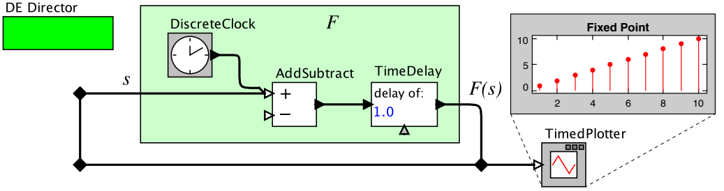
Figure 7.7: An example used to illustrate the Matsikoudis construction.
