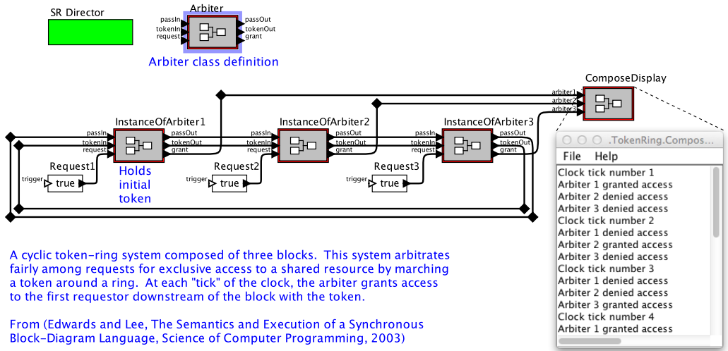
Figure 6.7: A token ring implementation in Ptolemy II from Edwards and Lee (2003a).
