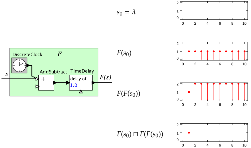
Figure 7.8: The Matsikoudis construction for the example in Figure 7.7.
