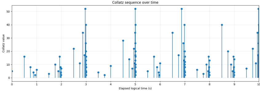
Figure 7.6: A plot of the signal that will be Zeno if the Collatz conjecture is false.
