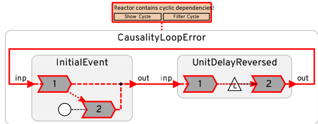
Figure 8.7: Causality loop error reported by the Lingua Franca validator.
