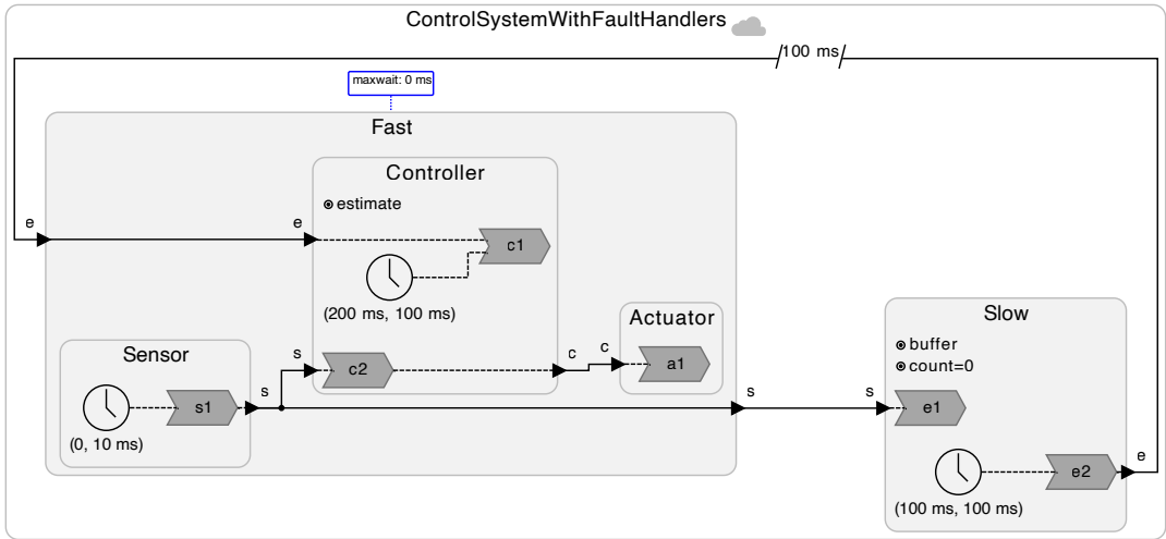
Figure 8.19: Control system with fault handlers.
