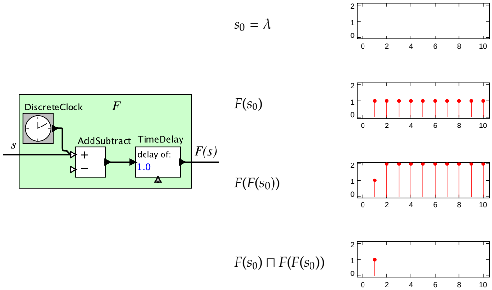
Figure 7.10: The Matsikoudis construction for the example in Figure 7.9.
