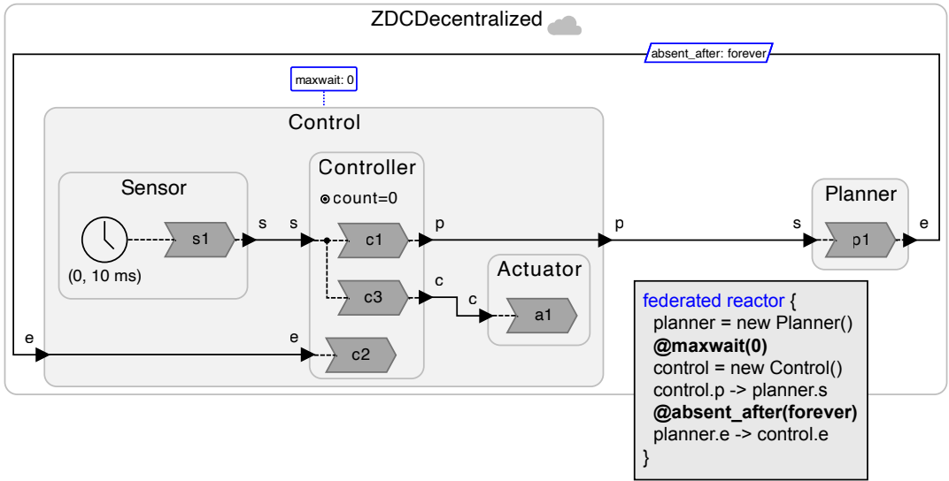
Figure 8.21: Zero-delay cycle with maxwait and absent_after offsets.
