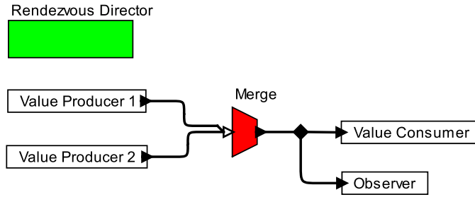
Figure 4.16: Observer pattern implemented in Ptolemy II's rendezvous domain.
