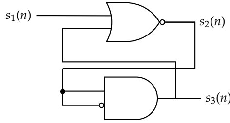
Figure 6.12: Non-constructive circuit with a single fixed point from Malik (1994).
