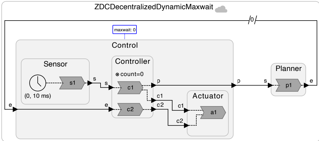
Figure 8.20: Microstep delay cycle with dynamic maxwait adjustment.
