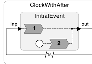
Figure 8.5: Simpler clock generator using an after delay instead of a unit delay reactor.
