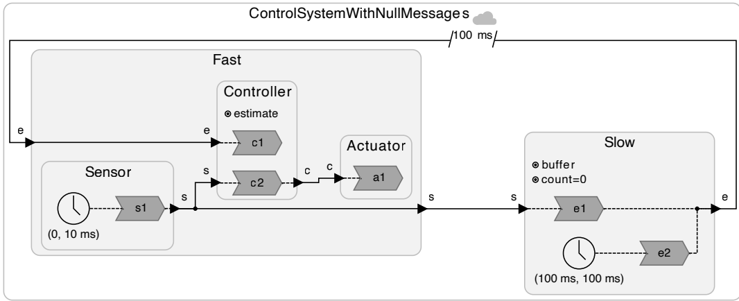
Figure 8.18: Decentralized coordination with null messages.
