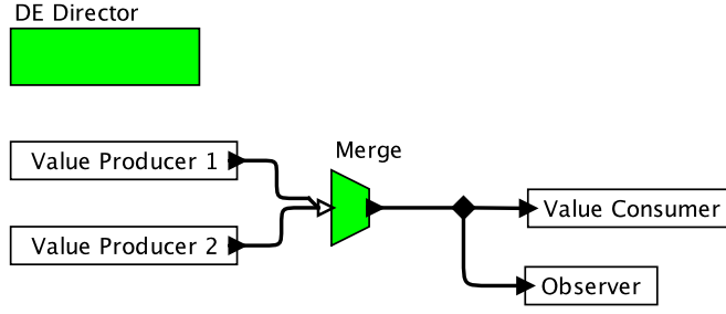
Figure 7.1: Observer pattern implemented in Ptolemy II's discrete-event domain.
