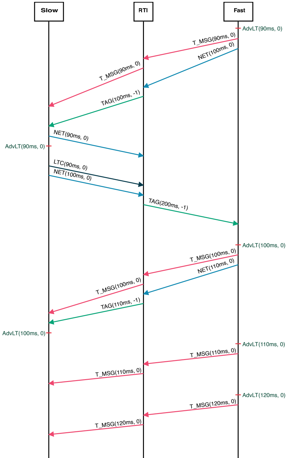
Figure 8.15: Trace of messages between federates and the RTI in a centralized coordination system. This diagram is automatically generated by the Lingua Franca tools.
