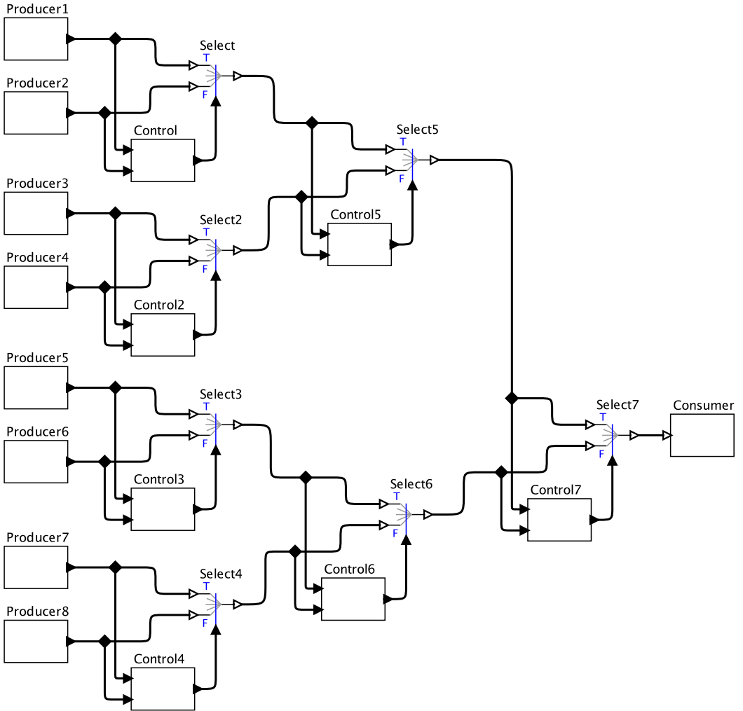
Figure 3.6: A variant of the program in Figure 3.4 that merges 8 sources rather than two.
