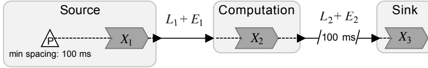
Figure 2.5: Three node system where a source sends a message through a computation with a logical execution time to a destination sporadically.
