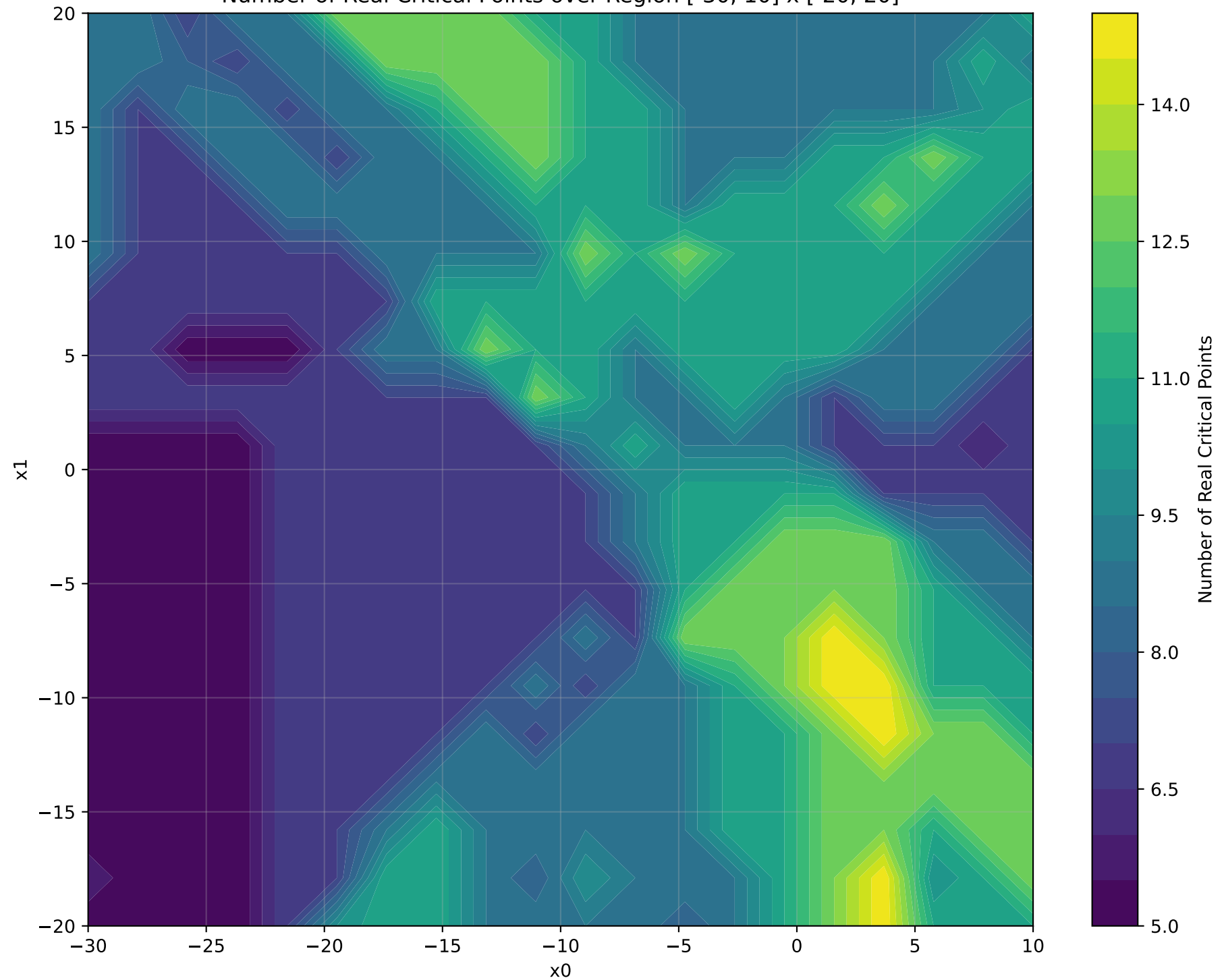
Number of Real Critical Points over Region [-30, 10] \times [-20, 20]
