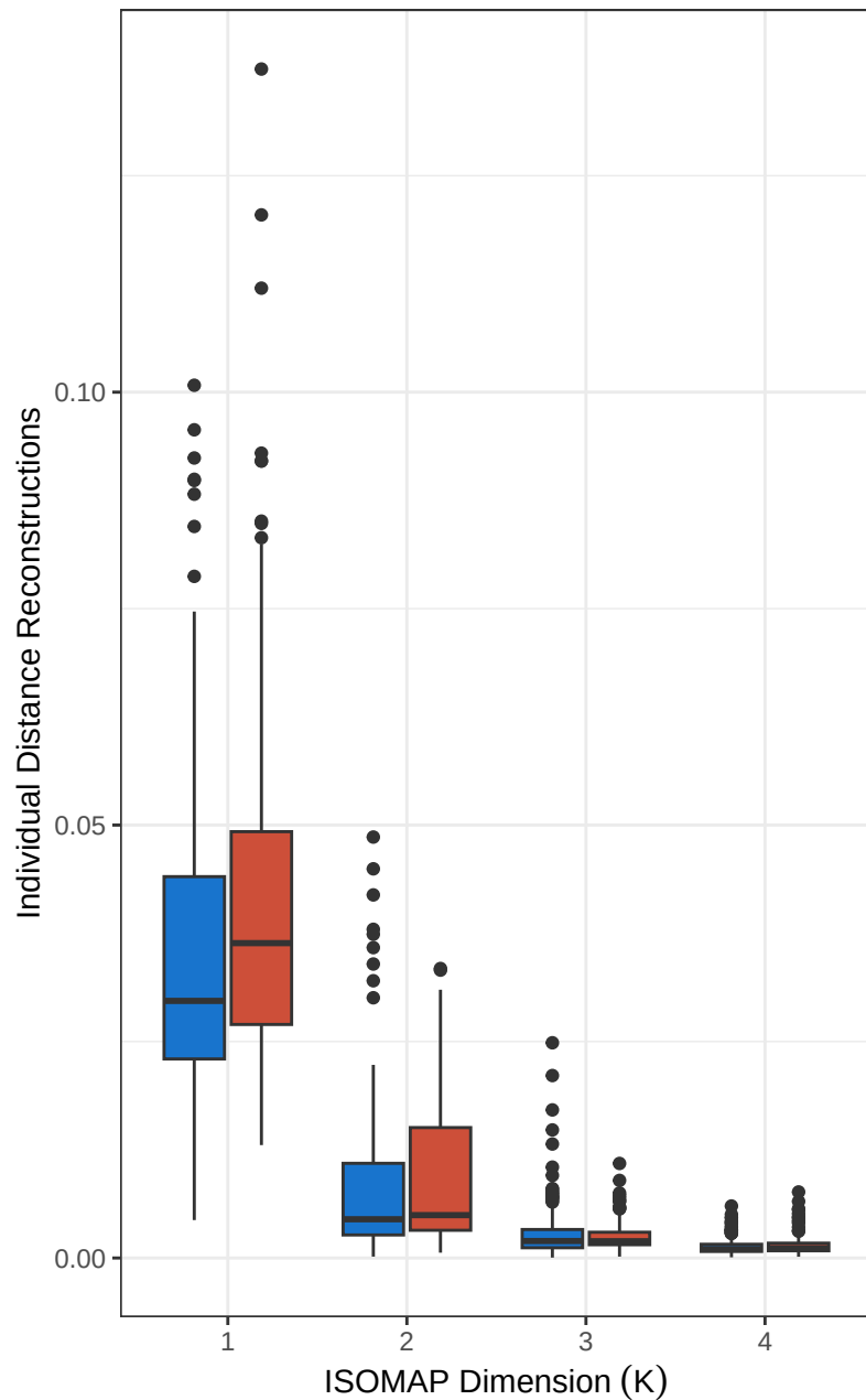
Individual Distance Reconstructions for Skew-normal
