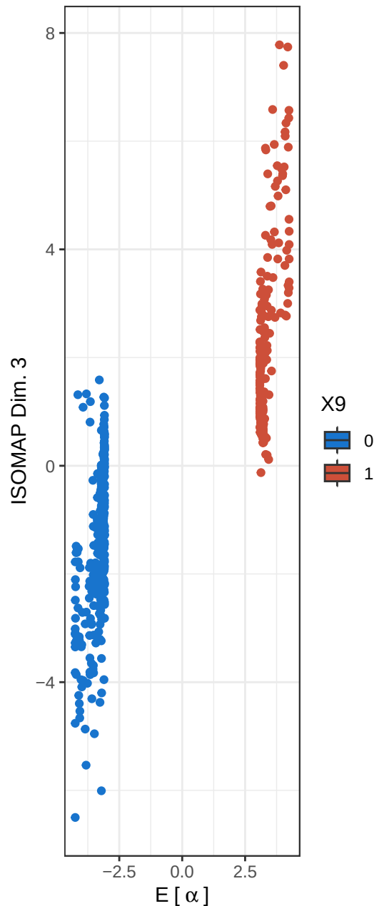
Third ISOMAP Dimension
