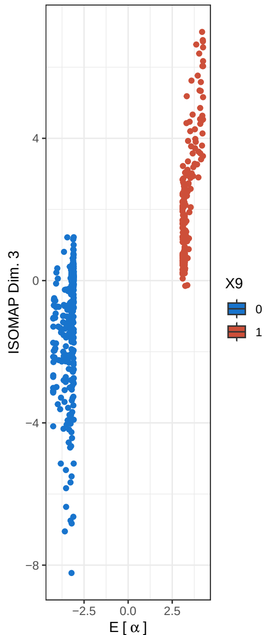
Individual Distance Reconstructions for Skew-normal Third ISOMAP Dimension
