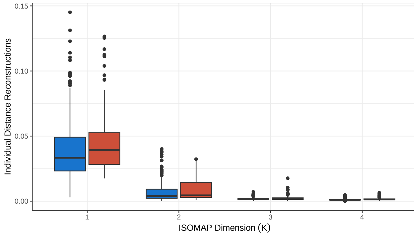
Individual Distance Reconstructions for Skew-normal Example
