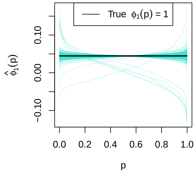
First Eigenfunction
