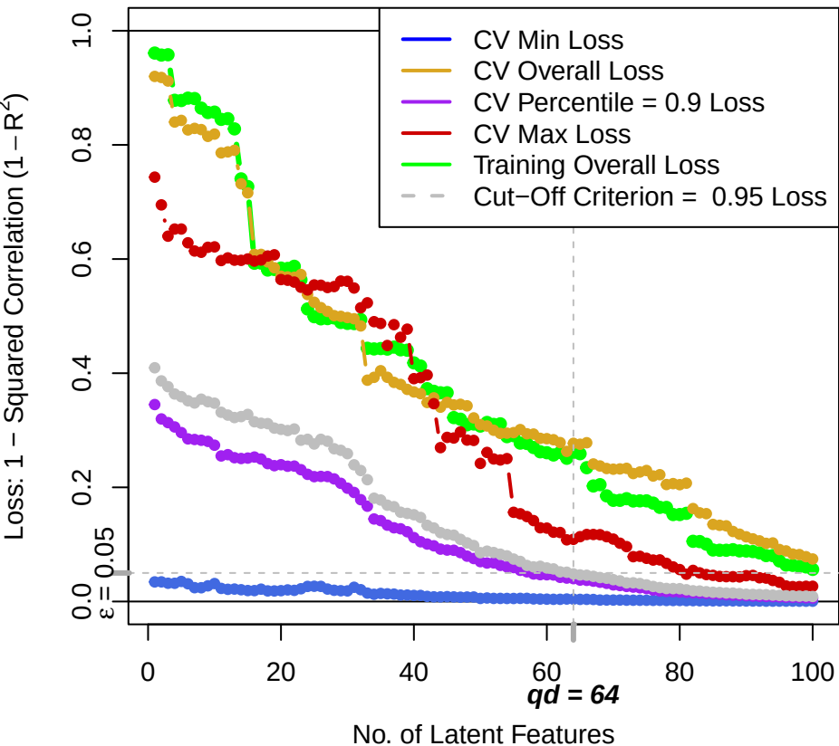
Latent Feature Representation Summary: MV-FPCA: max loss
