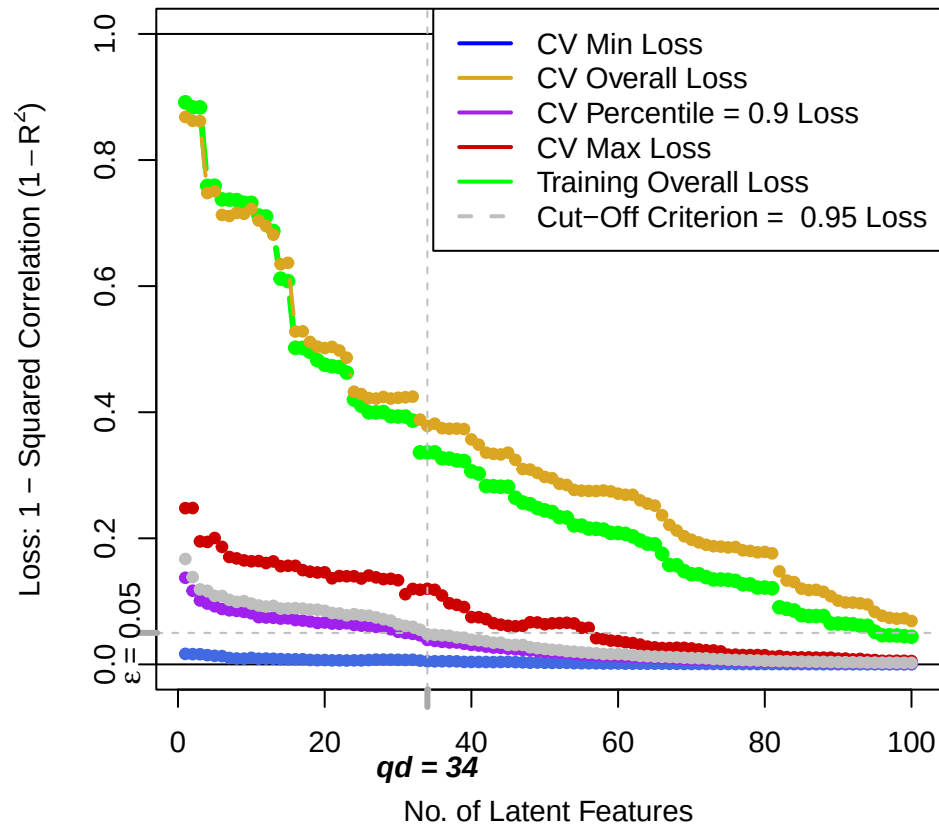
Latent Feature Representation Summary: MV-FPCA: mean loss
