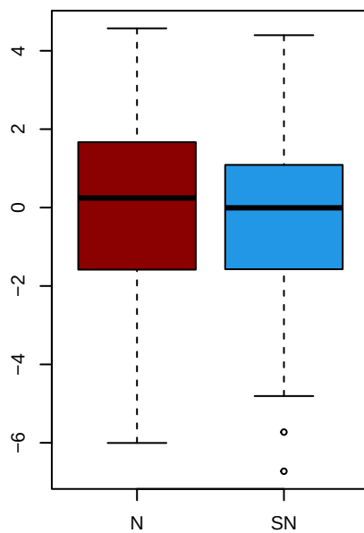
Log of Variances
