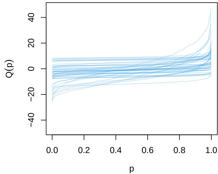
(b) Dataset from Skew-normal Group
