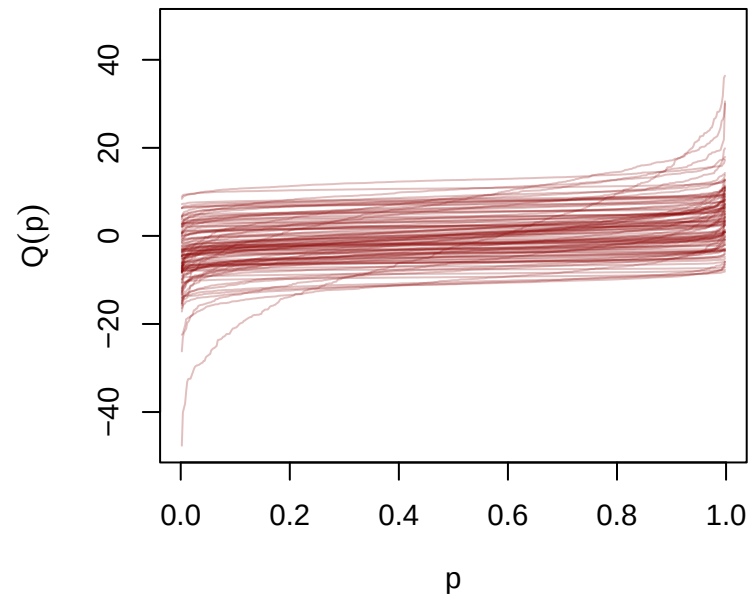
(a) Dataset from Normal Group
