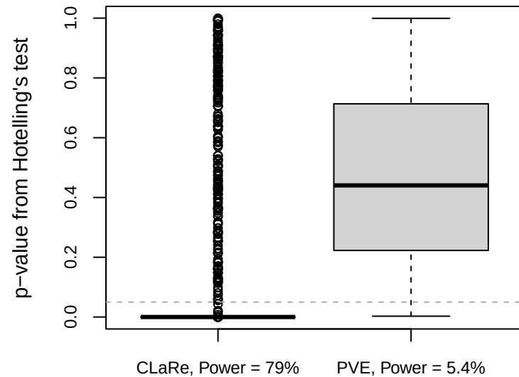
(c) Boxplot of p-values from Simulation
