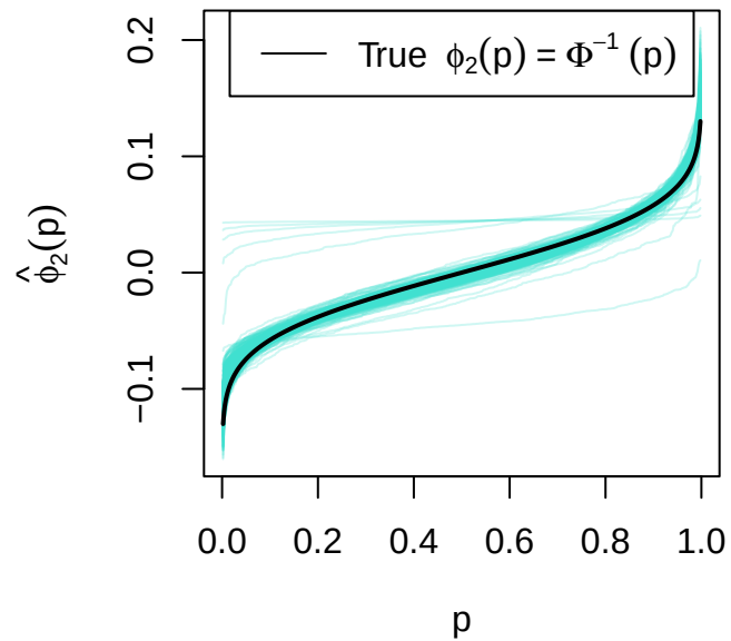
(e) Second Eigenfunction
