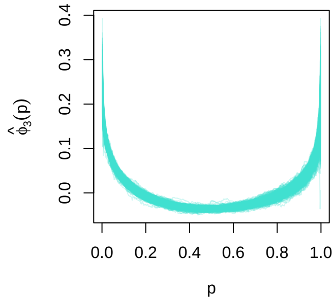
(f) Third Eigenfunction
