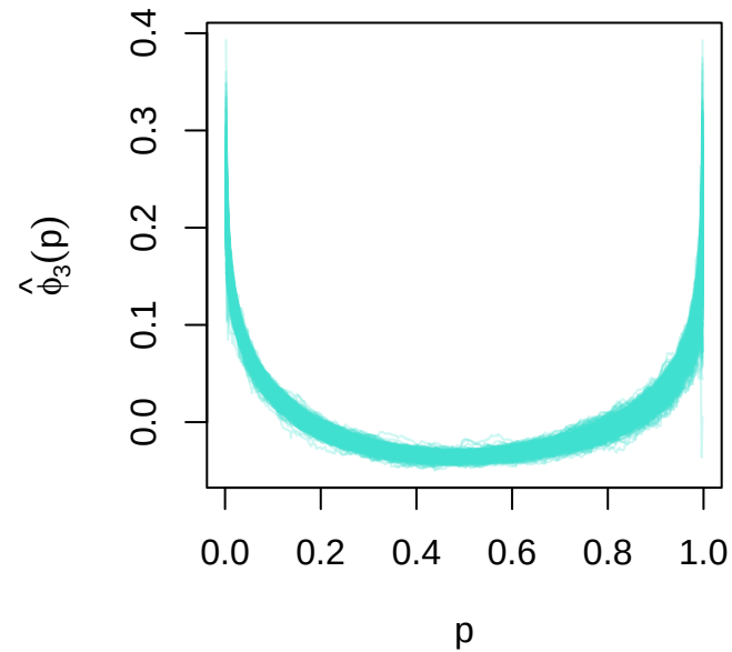
Third Eigenfunction
