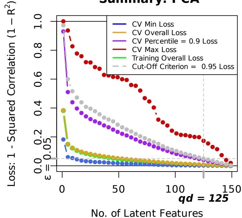
Latent Feature Representation Summary: PCA
