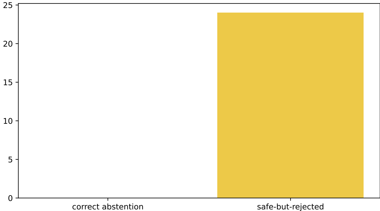
Abstention attribution
