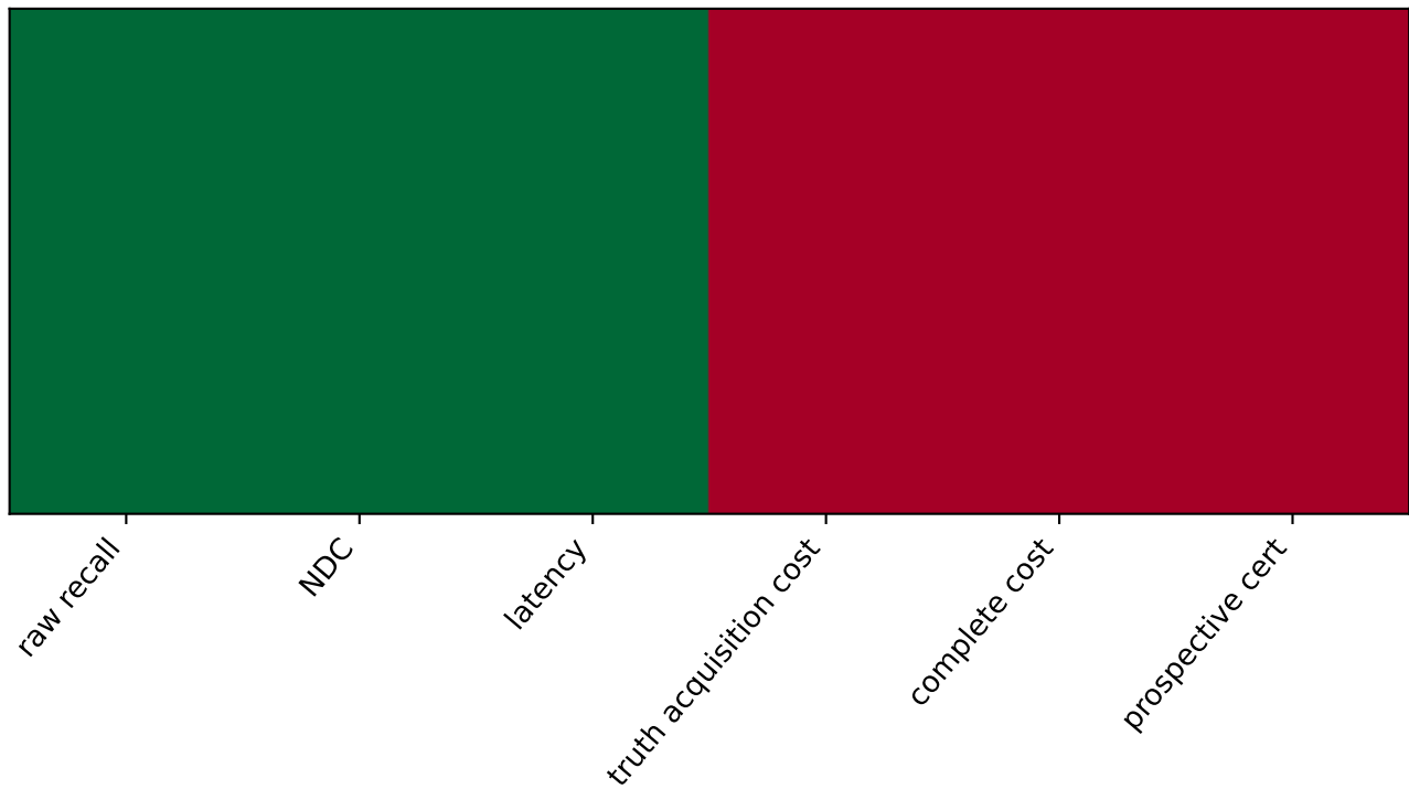
Estimability matrix
