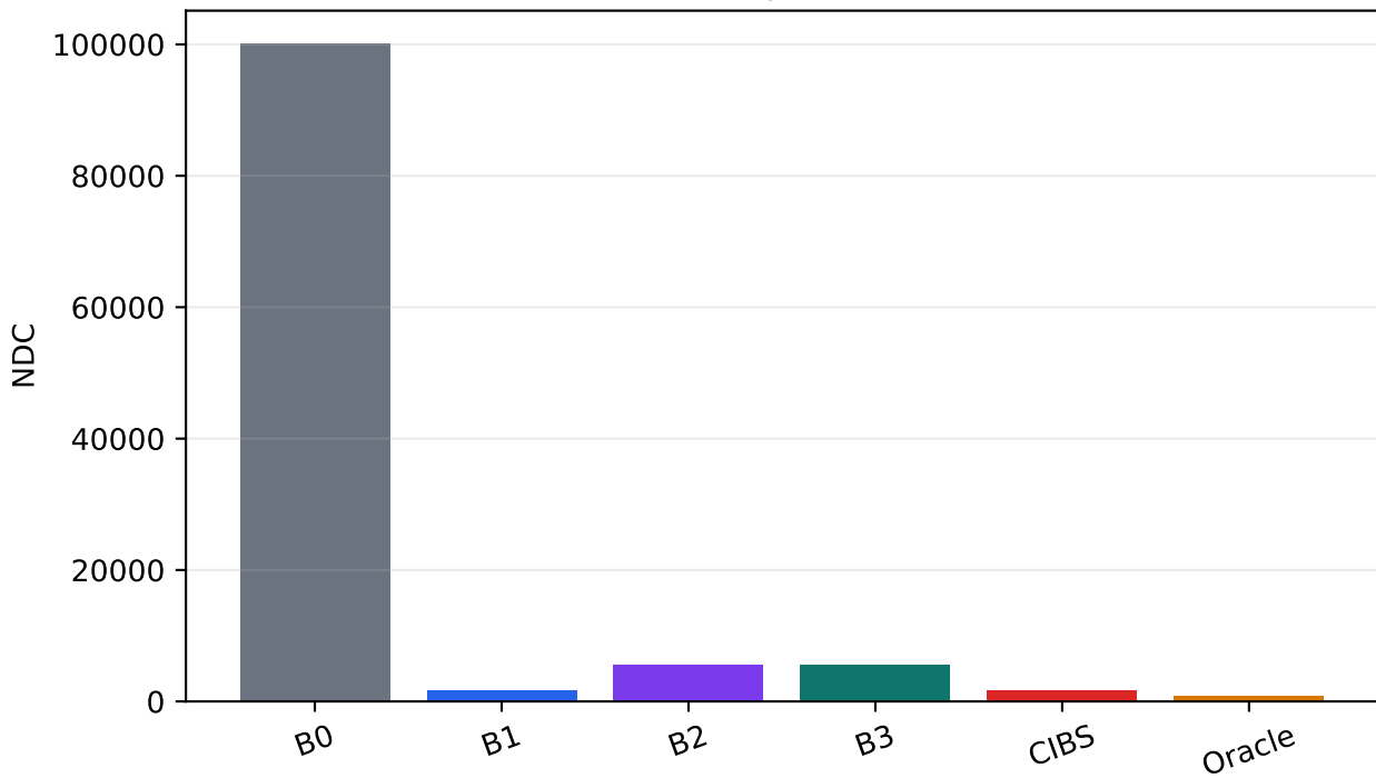
SIFT-100K — p95 exact NDC
