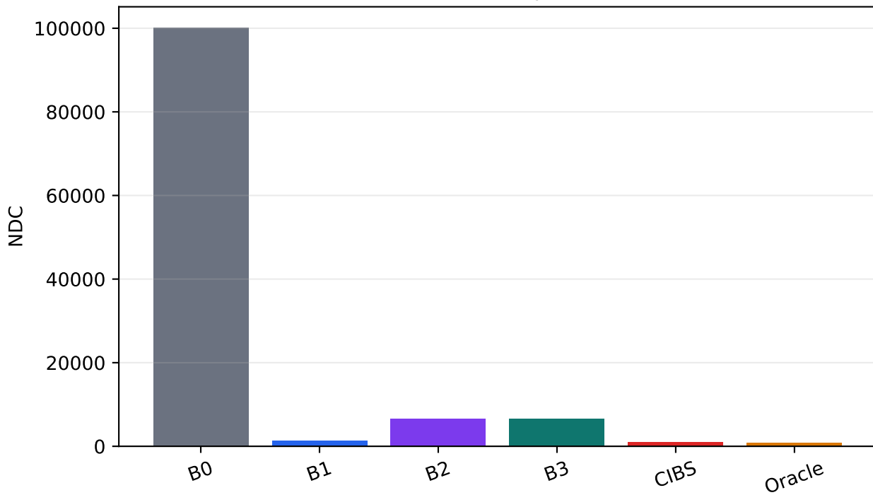
ArXiv-Nomic-100K — p95 exact NDC
