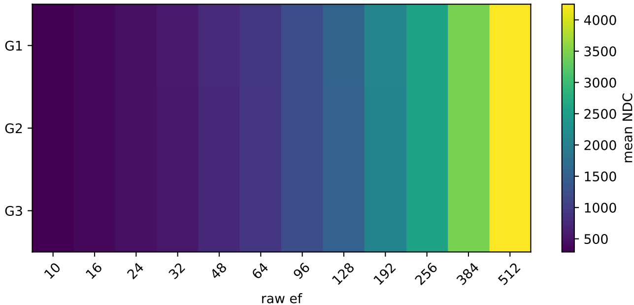
SIFT-100K — sentinel mean NDC by build
