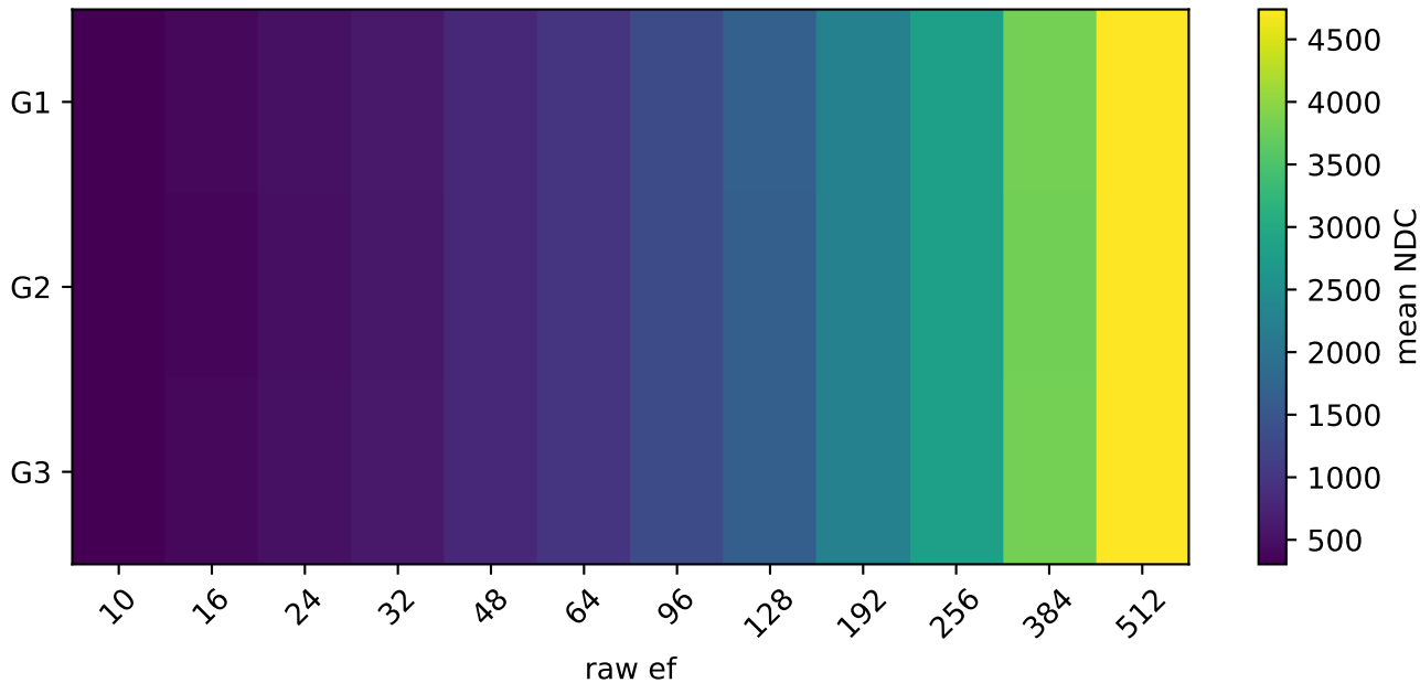
ArXiv-Nomic-100K — sentinel mean NDC by build
