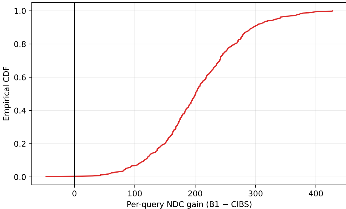
ArXiv-Nomic-100K — paired evaluation gain
