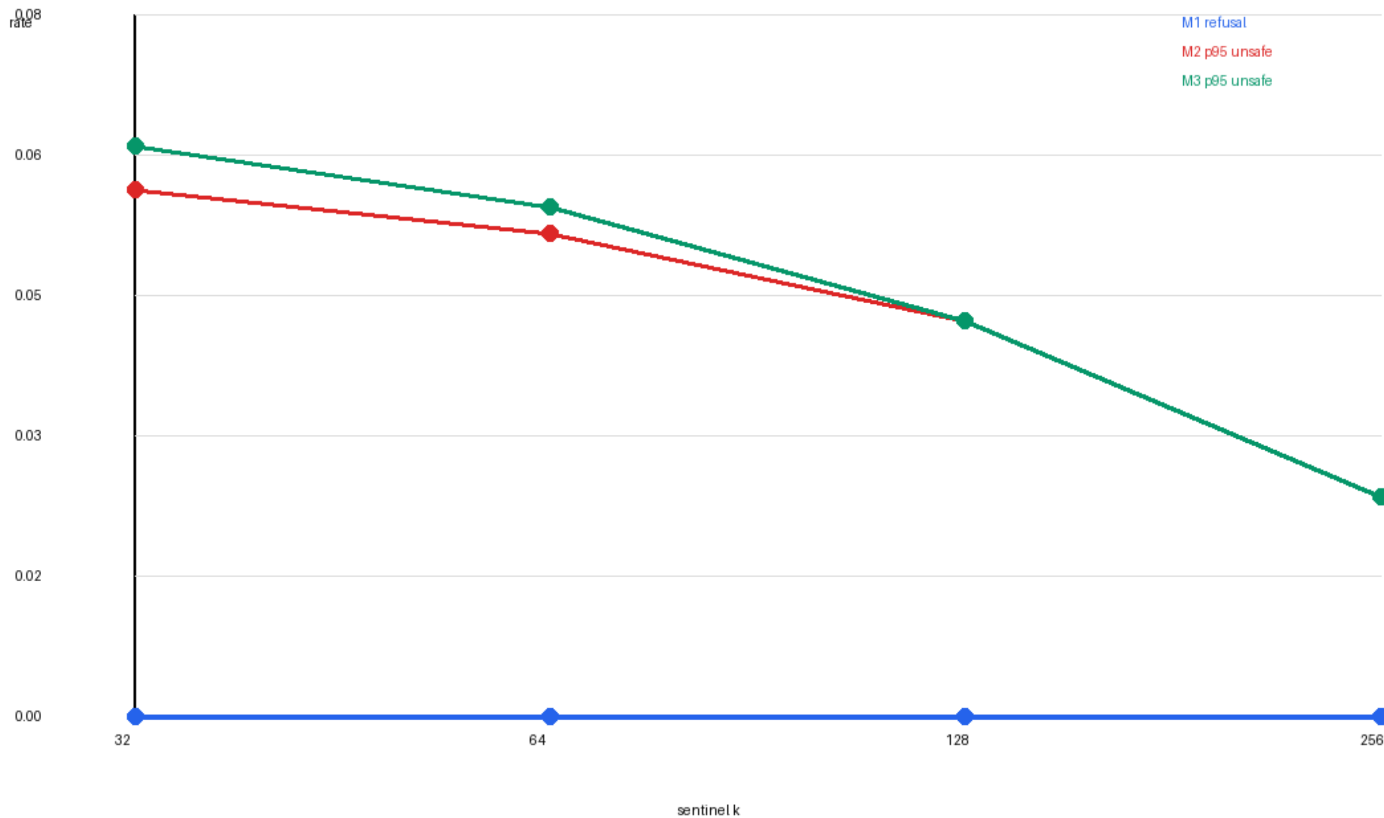
Refusal versus unsafe accept
