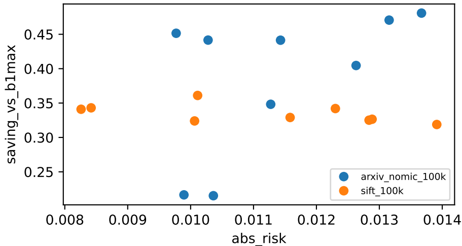
target_build_forest
