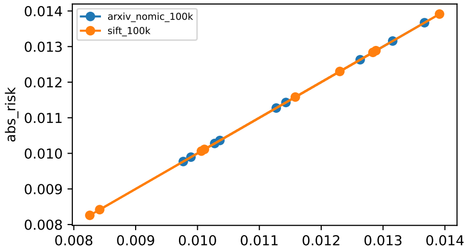
build_meta_risk
