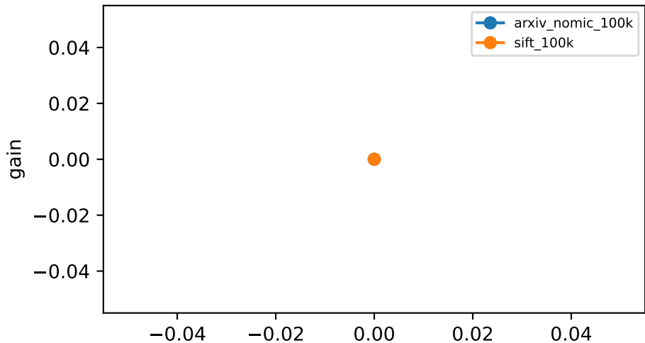
early_signal
