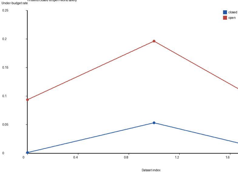
hnsplib closed vs open-world safety
