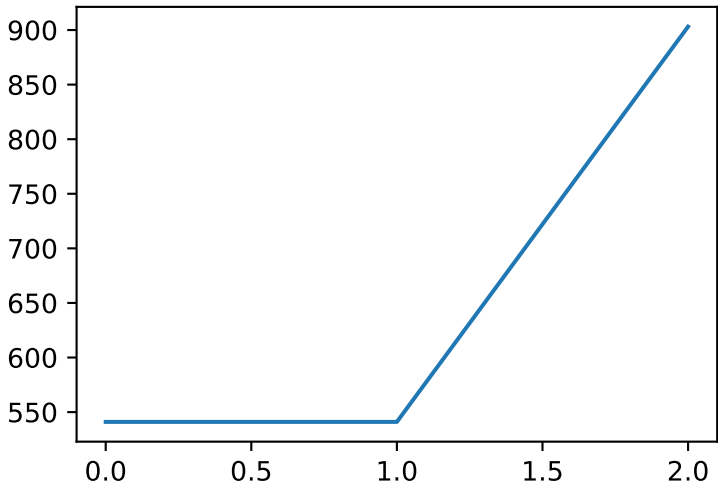
cost_pareto
