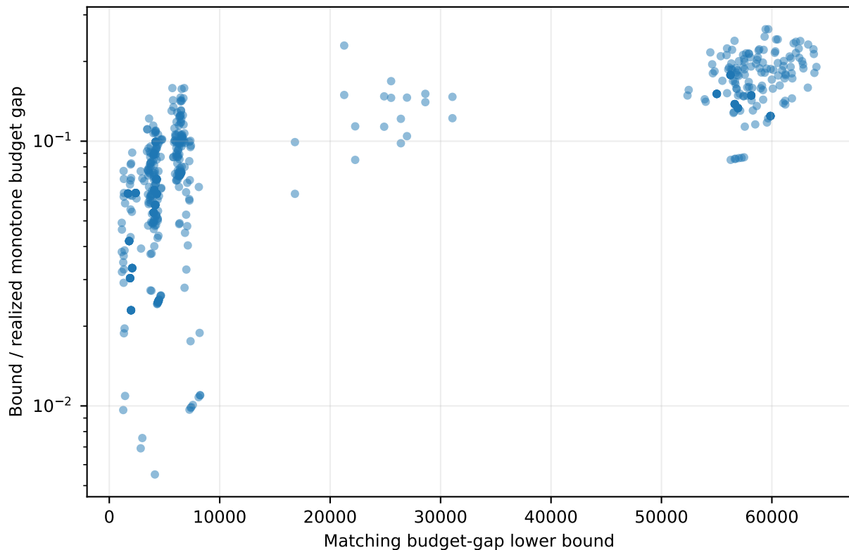
Matching lower-bound tightness (computational; T4 proof sketch)
