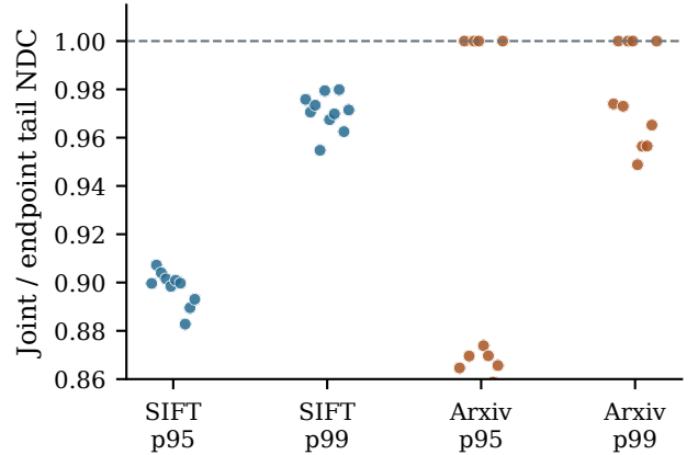
Figure 5: Per-target tail ratios for joint-error replay, relative to that target’s endpoint; ten dots per dataset/quantile. Equality reflects an endpoint fallback. All ratios are at most one. These descriptive tail comparisons are not formal non-inferiority certificates or wall-clock results.
