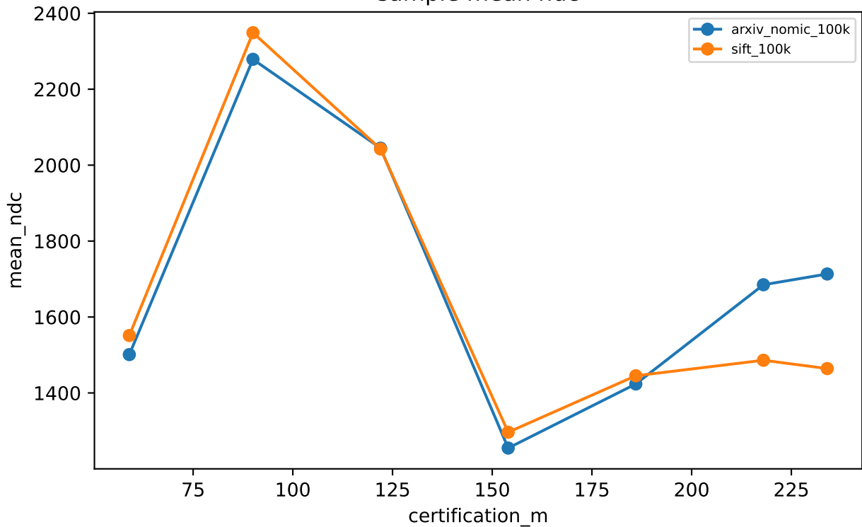
sample mean ndc
