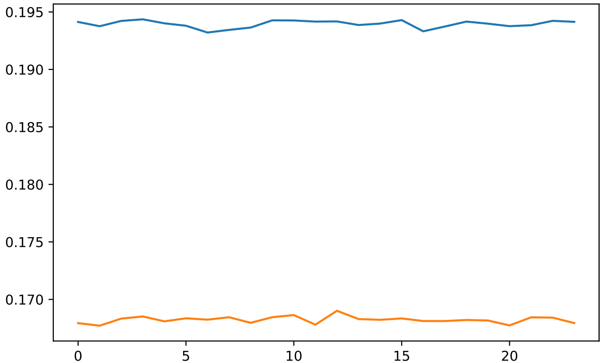
LOBO robustness
