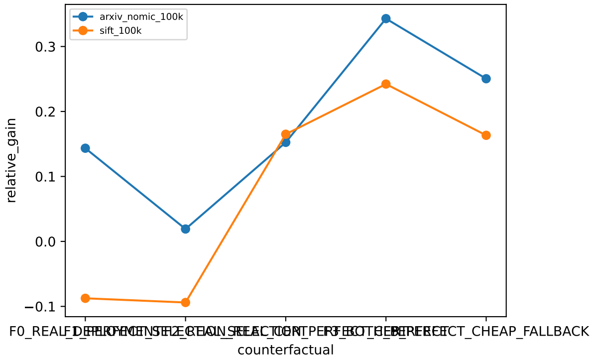
named gain
